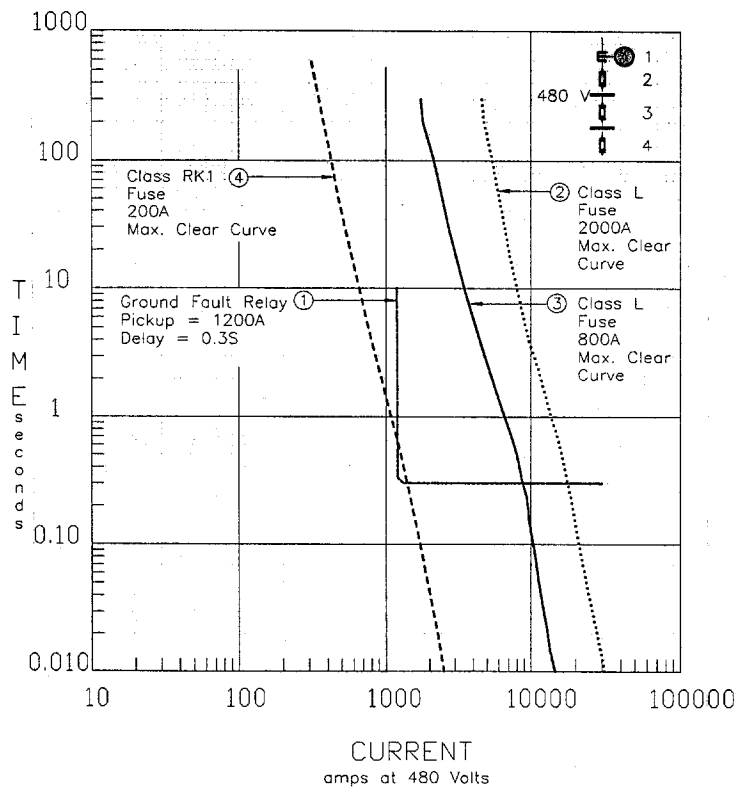
FIGURE 5 - FUSED MAIN AND FEEDERS, GROUND PROTECTION ON MAIN ONLY Qual-Tech Engineers, Inc.
