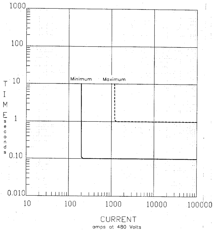
FIGURE 1 - GROUND FAULT SETTING LIMITS FOR 2000A MAIN Qual-Tech Engineers, Inc.
