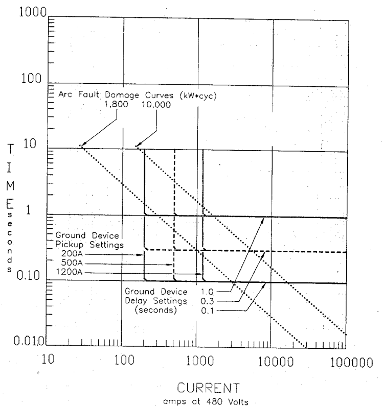
FIGURE 2B - GROUND FAULT SETTINGS VERSUS ARC FAULT DAMAGE LEVELS Qual-Tech Engineers, Inc.
