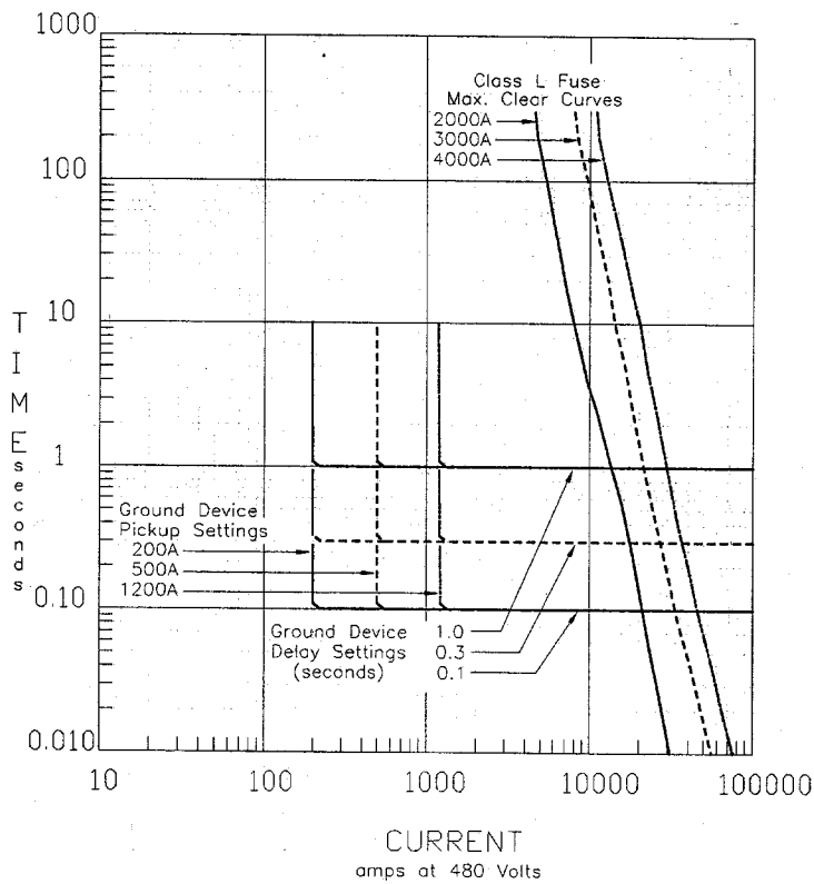
FIGURE 3 - GROUND FAULT SETTINGS VERSUS TYPICAL MAINS FUSING Qual-Tech Engineers, Inc.
