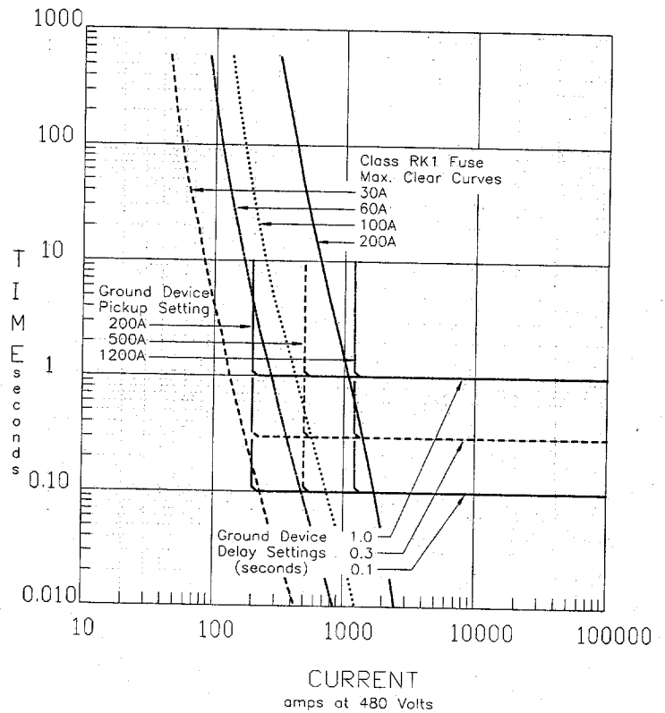
FIGURE 4 - GROUND FAULT SETTINGS VERSUS TYPICAL BRANCH FUSING Qual-Tech Engineers, Inc.
