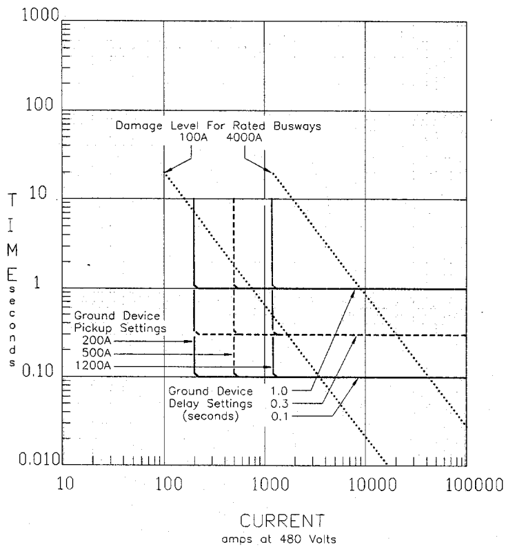
FIGURE 2A - GROUND FAULT SETTINGS VERSUS BUSWAY DAMAGE LEVELS Qual-Tech Engineers, Inc.
