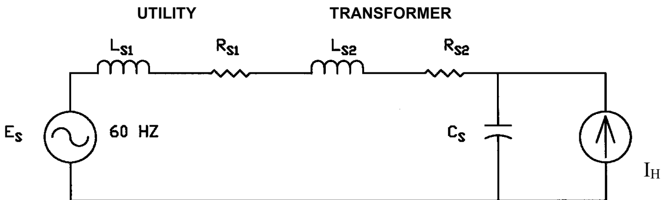
Figure 2: Simplified Circuit Model
