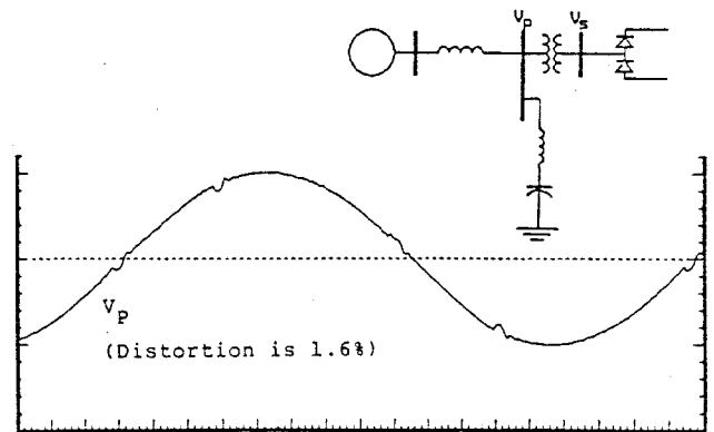
Fig. 11 Adding a Filter Capacitor Bank
