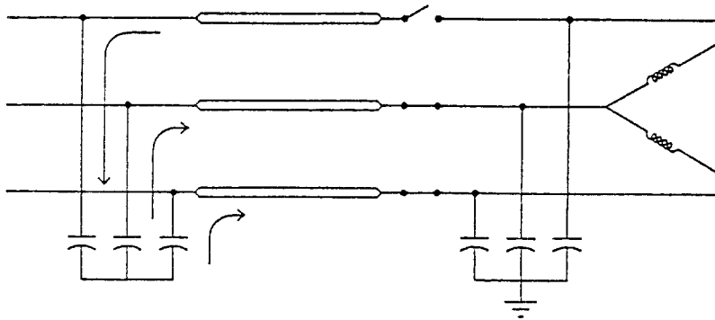
Virtual Current Chopping Circuit
